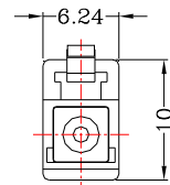
LC BOA Double Latch
